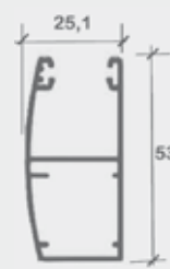
H25C (curva)
